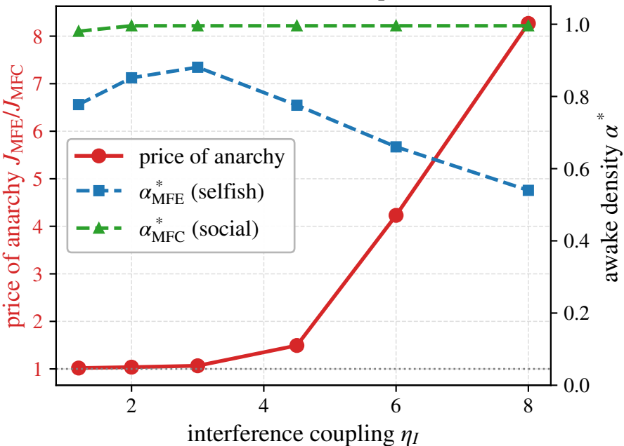
Coordination collapse
