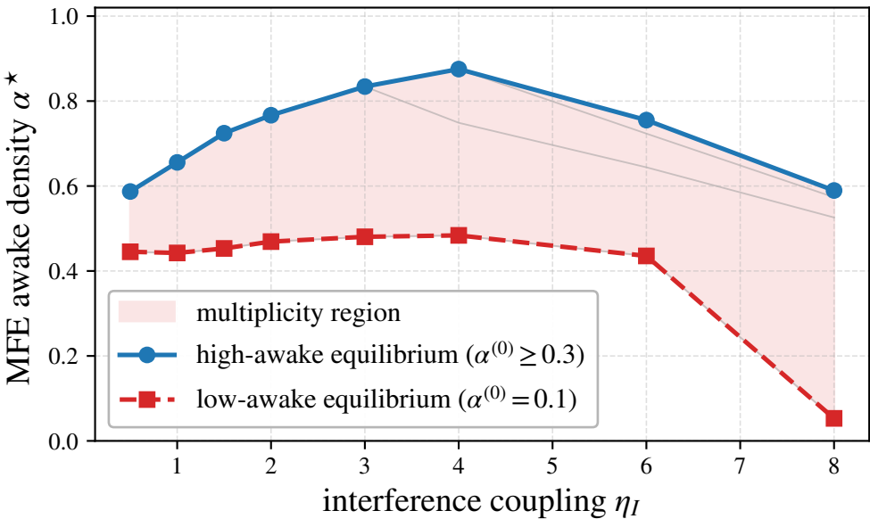
Equilibrium bifurcation (milan, N=100 )
