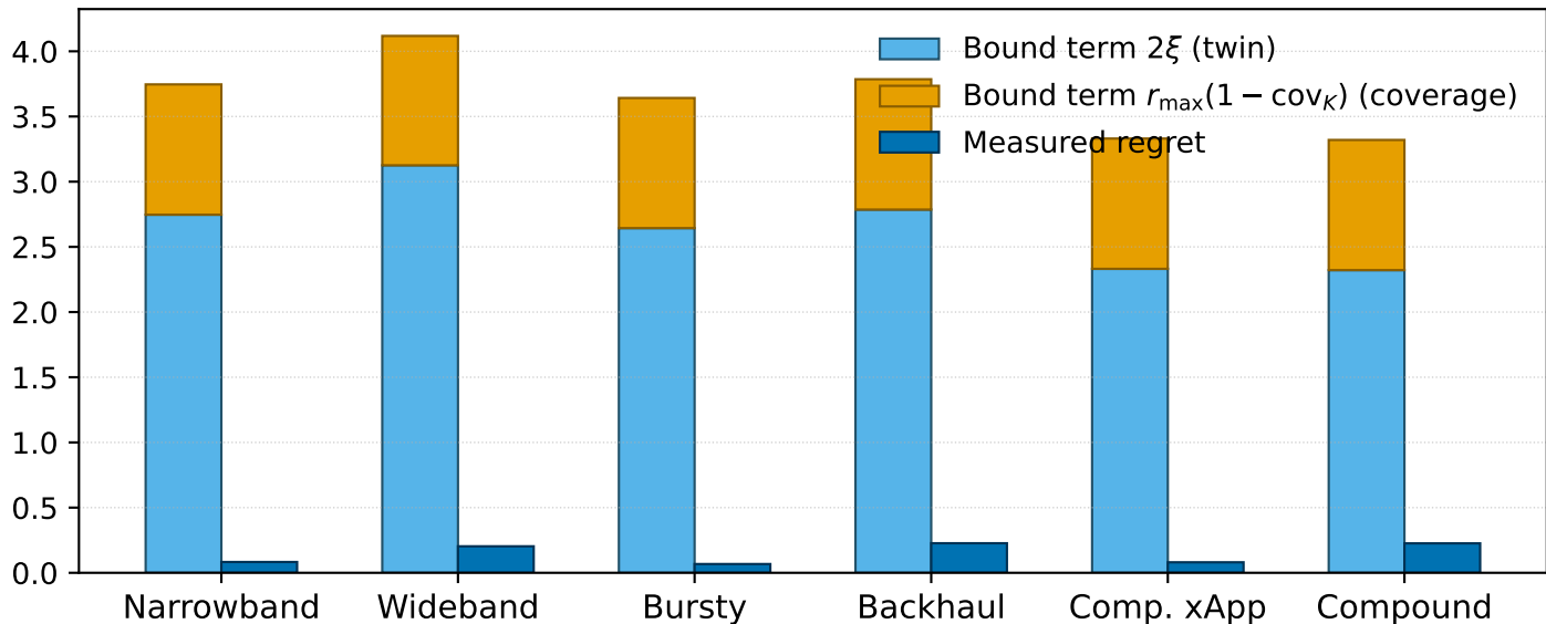
Per-cycle regret
