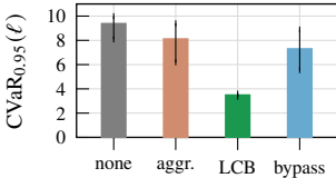
filter variant
