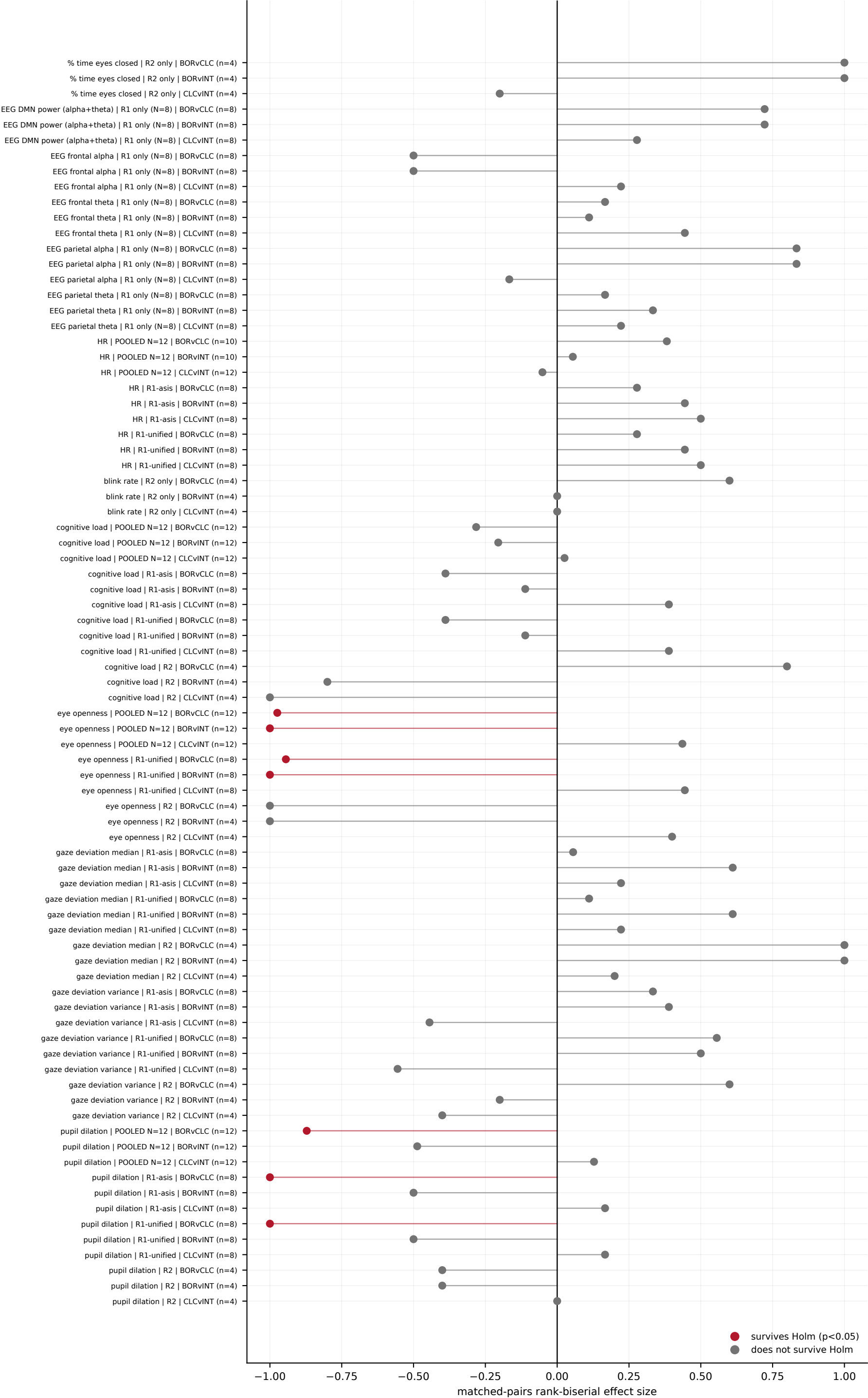
Effect sizes, all 81 pairwise contrasts (7 survive Holm at alpha=0.05)
