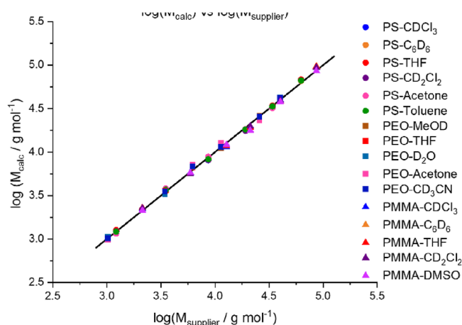
Figure 4. Calculated molar masses via Equation (12) with the parameters of Table 1 vs molar masses of the supplier for PS, PEO, and PMMA in different solvents at T = 298.15 K. The black line represents the molar masses M_{\text{supplier}} .
