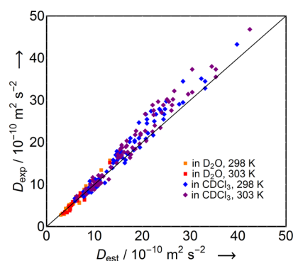
Figure 3. Measured diffusion coefficient plotted against diffusion coefficient calculated using for 24 small molecules in D_2O at 298 K (filled yellow squares), 24 small molecules in D_2O at 303 K (filled red squares), 76 small molecules in CDCl_3 at 298 K (filled blue diamonds), and 76 small molecules in CDCl_3 at 303 K (filled purple diamonds). Data are drawn from ref .
