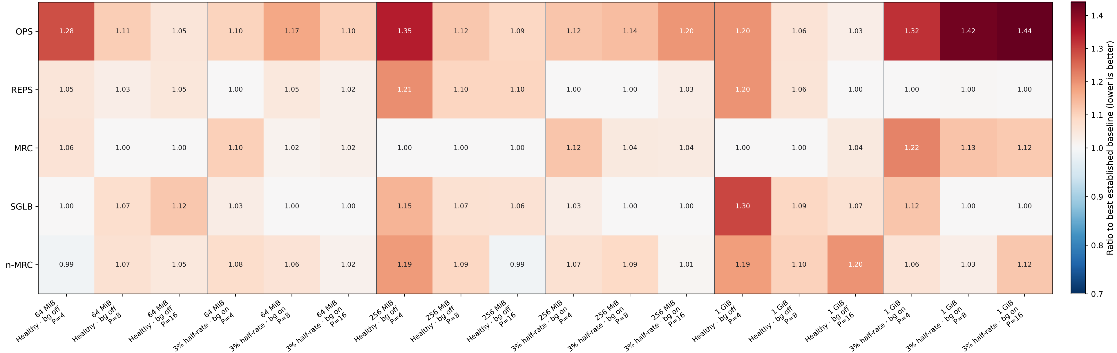
All-to-All CCT · 128 nodes · three-seed geometric mean MRC uses one-cycle no-rearm; lower is better
