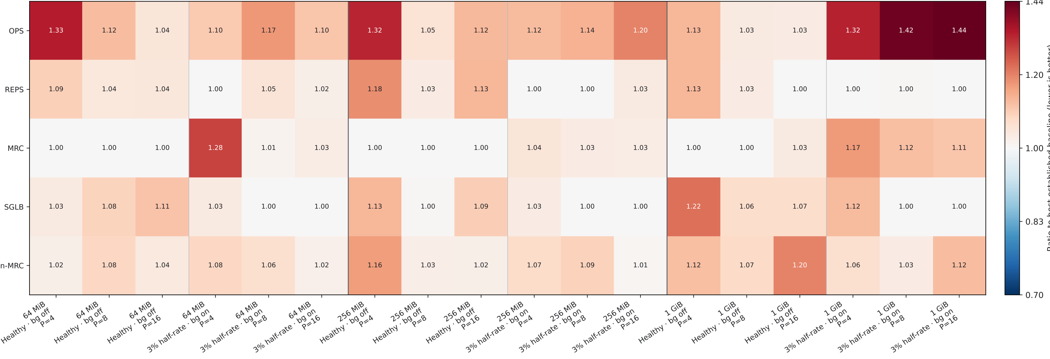
All-to-All CCT · 128 nodes · three-seed geometric mean Lower is better; columns group size, condition, and parallelism
