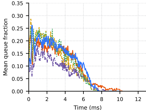
Mean Spine queue occupancy
