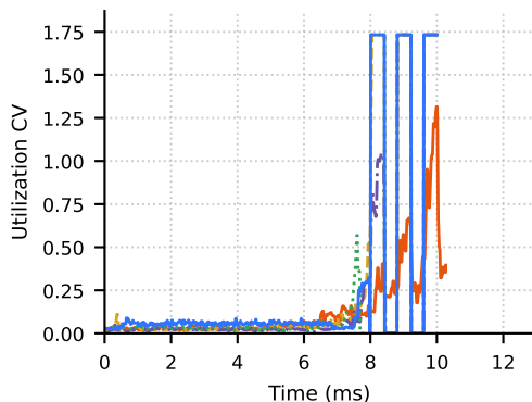
Spine utilization imbalance
