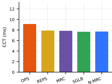
Three-seed collective completion
