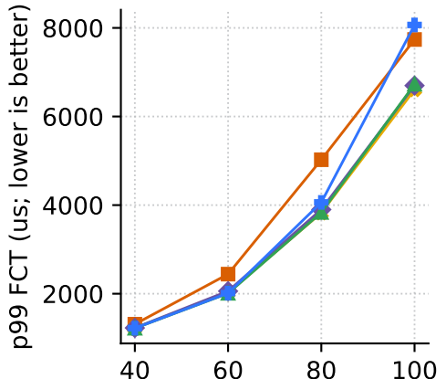
Asymmetric P2P: WebSearch
