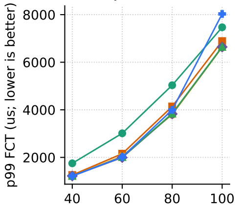
Healthy P2P: WebSearch
