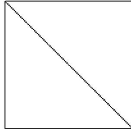
diag_neg_full (a = -1.00, b = 101.00)
