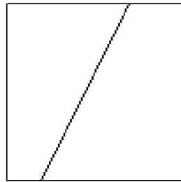
steep_shifted (a = 2.00, b = -40.00)
