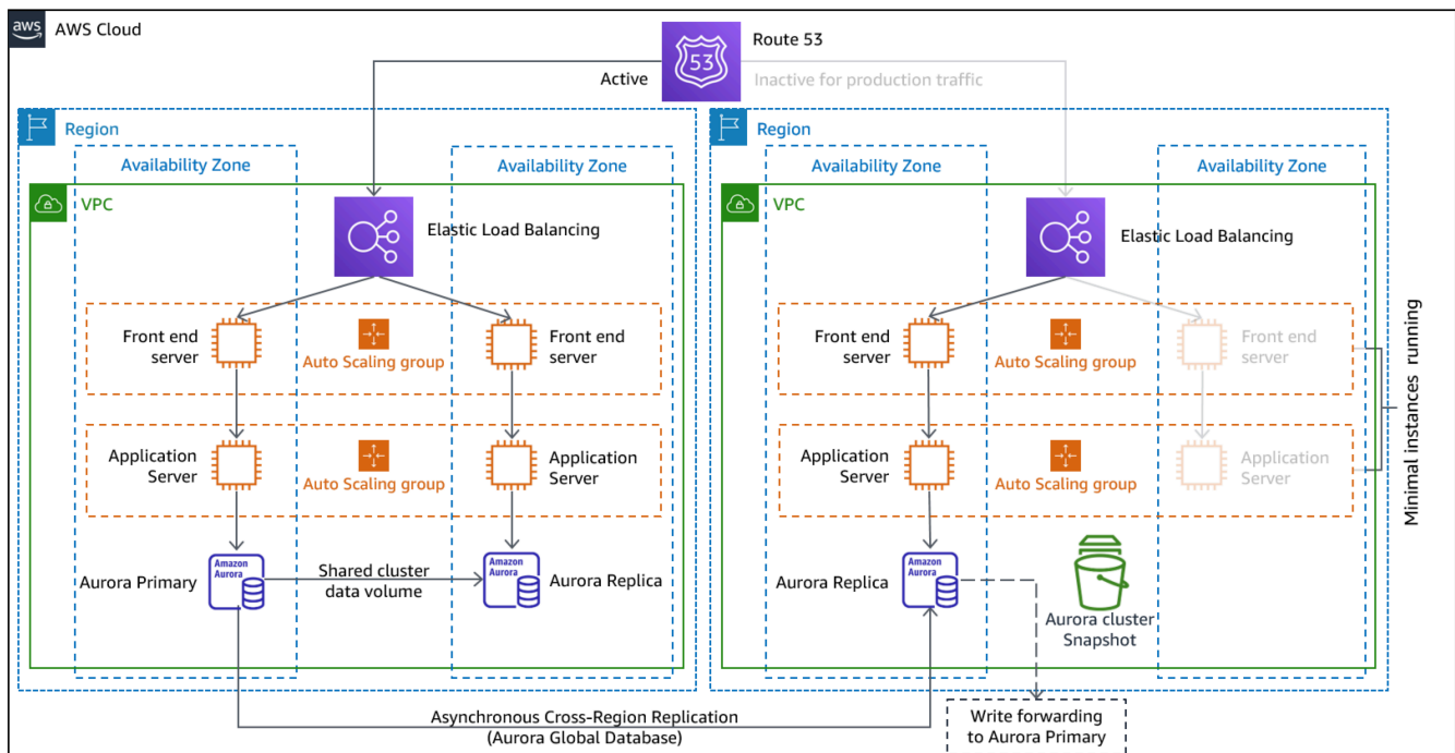
Figure 21: Warm standby architecture
