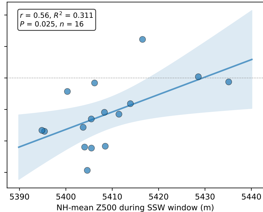
b Tropospheric circulation (Z500)
