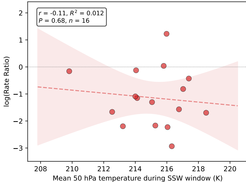
a Stratospheric intensity
