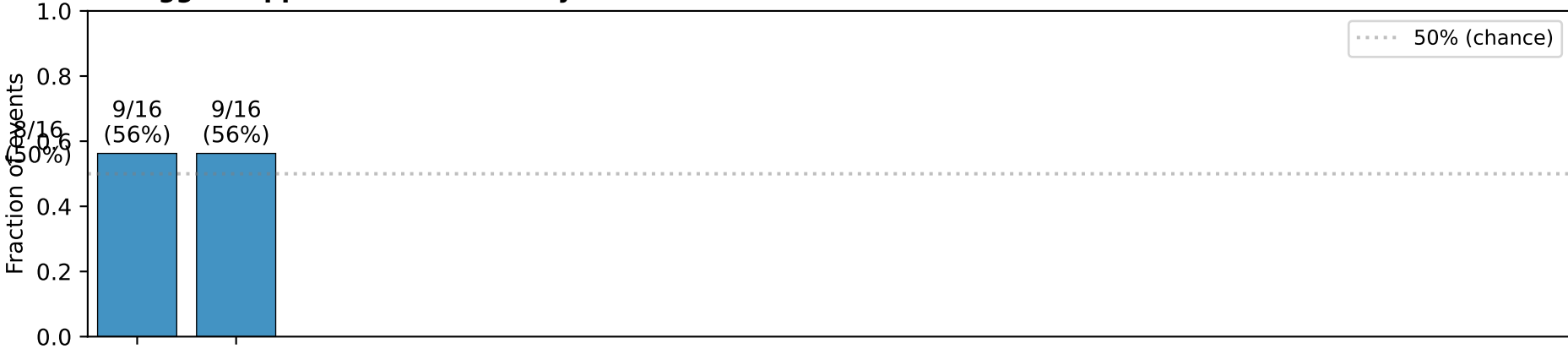
C Trigger suppression consistency across 16 events
