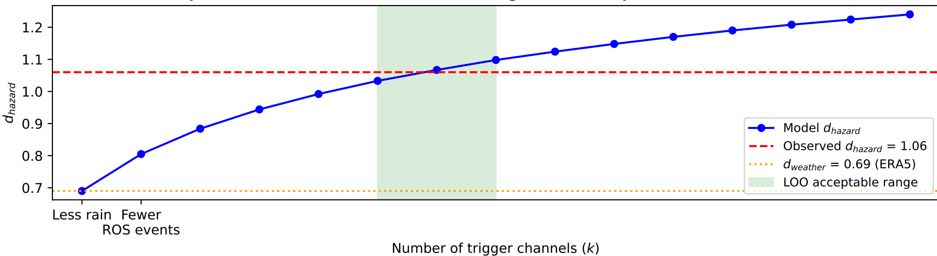
D Threshold amplification: modest weather shift → large hazard response
