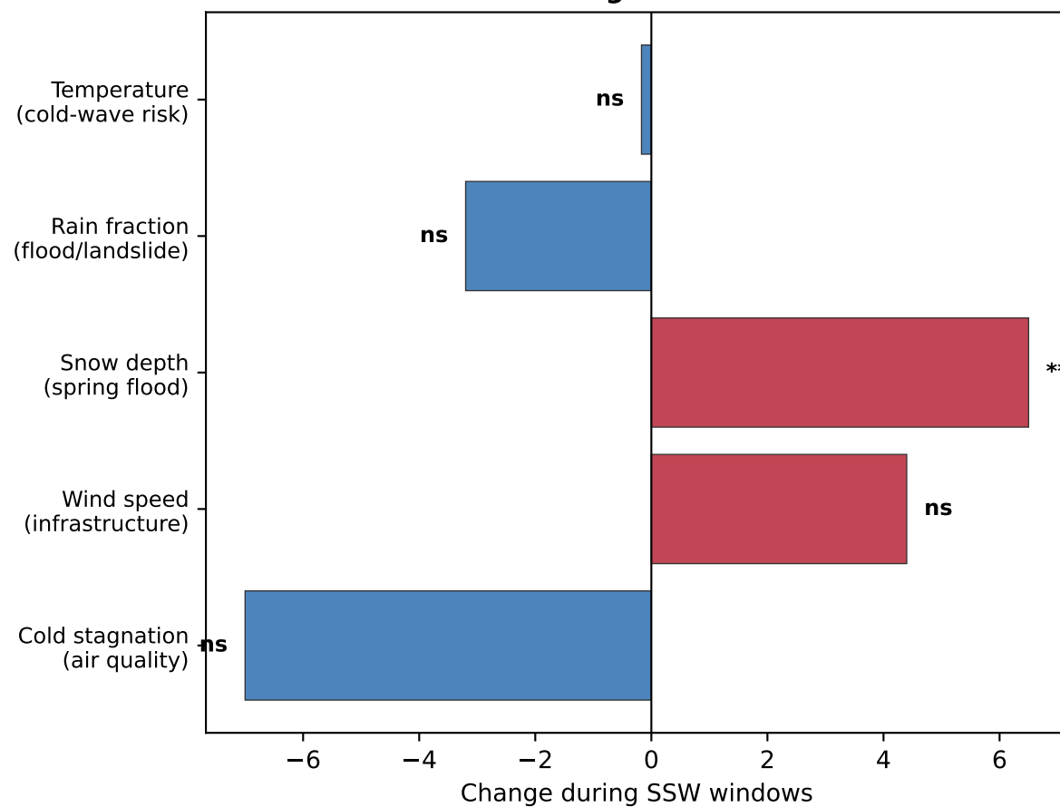
c Loaded-gun mechanism: decoupled loading-trigger
