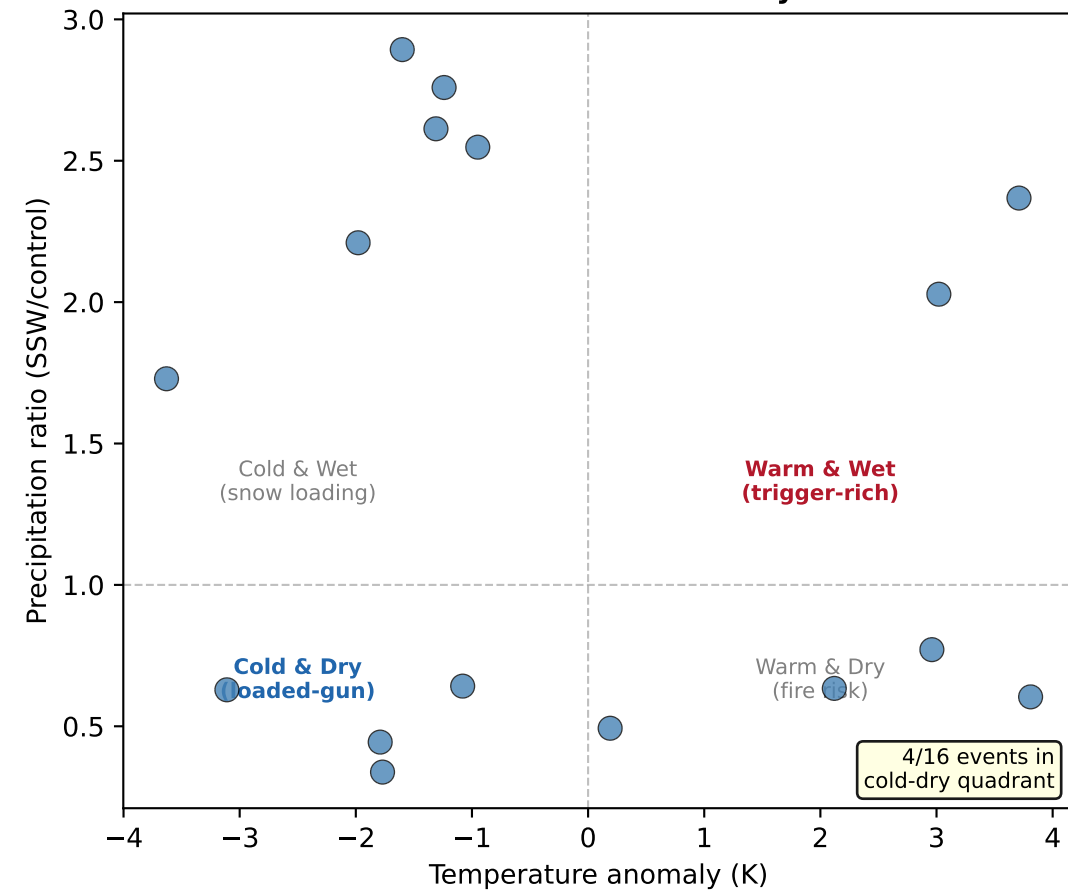
d Multi-hazard simultaneity per SSW event
