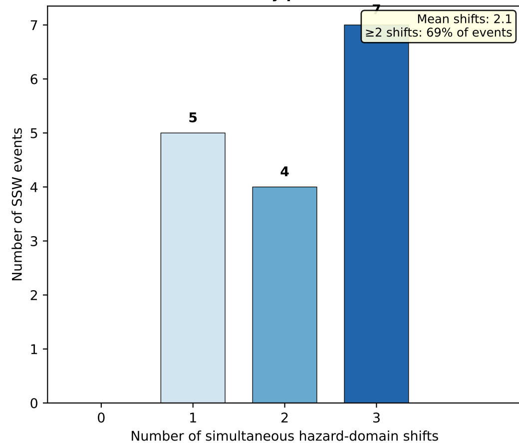
d Multi-hazard simultaneity per SSW event
