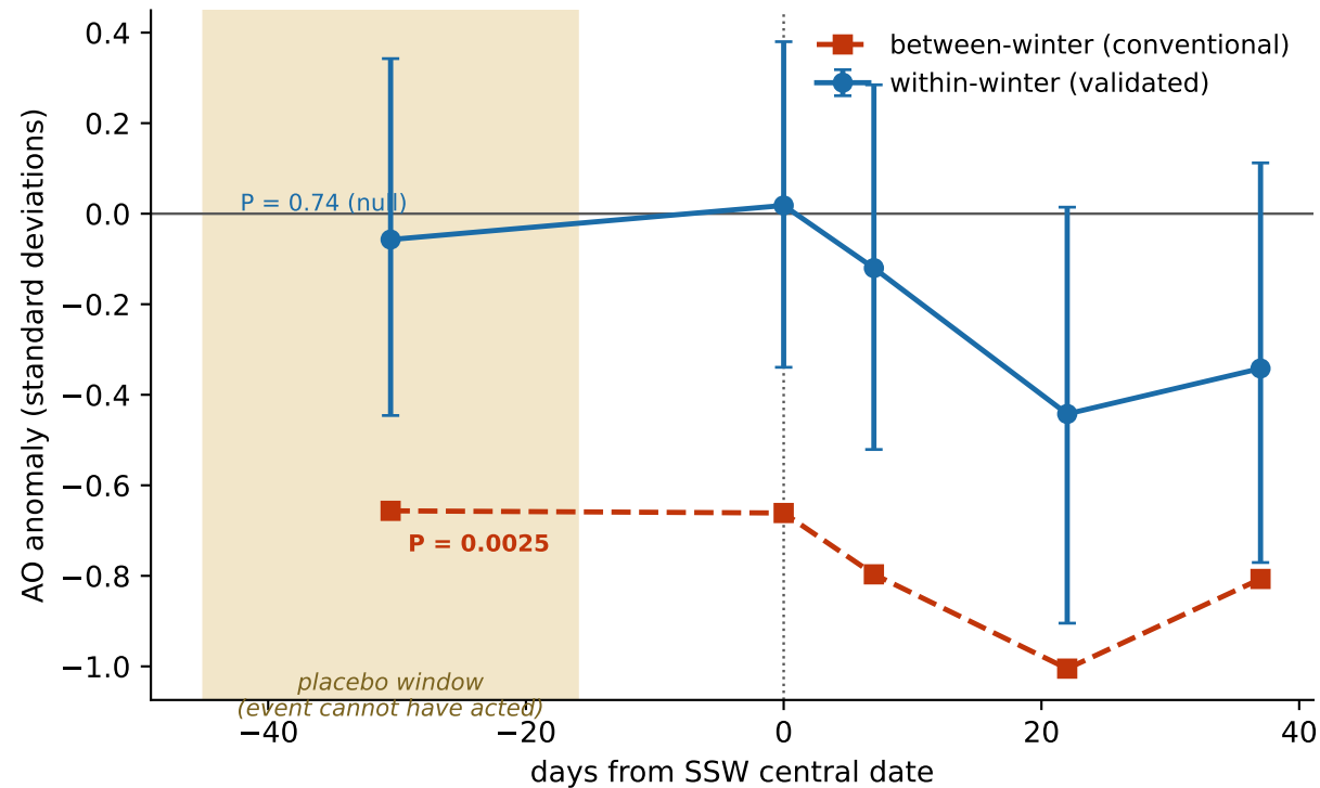
Arctic Oscillation response to 47 major SSWs, 1950–2026
