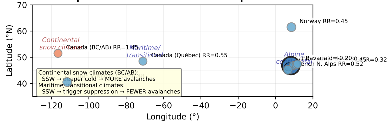
b Hemispheric Context: Climate-Zone Dependence
