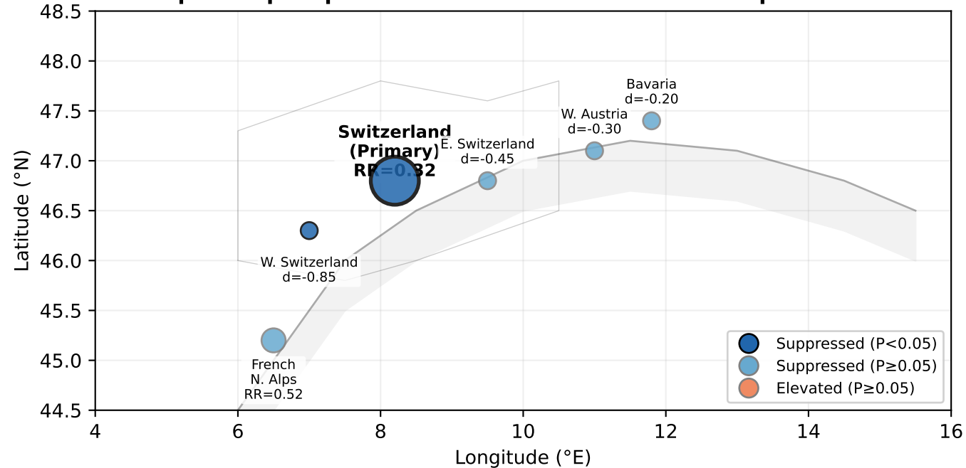
a European Alps: Spatial Pattern of SSW-Avalanche Response
