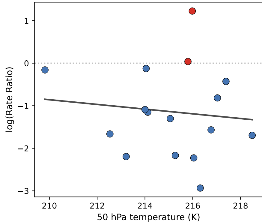
c Stratospheric dose (null) r = -0.11 , P = 0.683 , R^2 = 0.01
