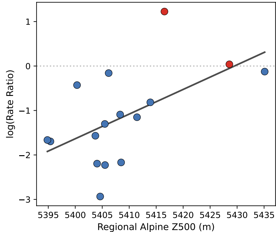
a Tropospheric dose r = 0.56 , P = 0.025 , R^2 = 0.31
