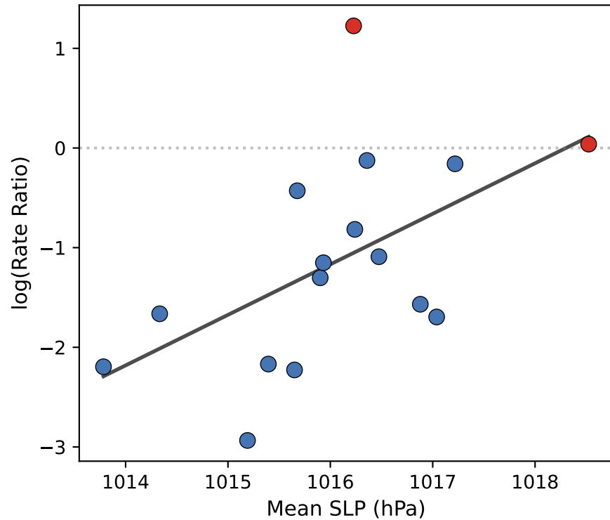
b Surface pressure dose r = 0.54 , P = 0.032 , R^2 = 0.29
