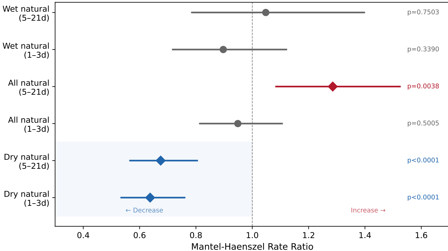
Figure 2: Dry Avalanche Specificity (Case-crossover, within winter×15-day strata)
