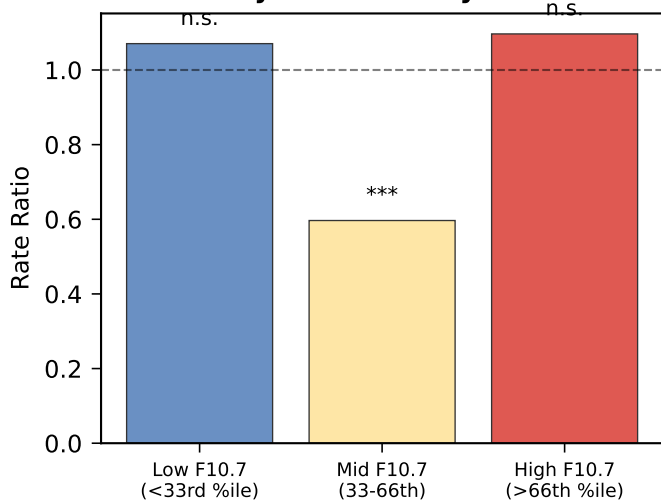
a Effect by solar activity level
