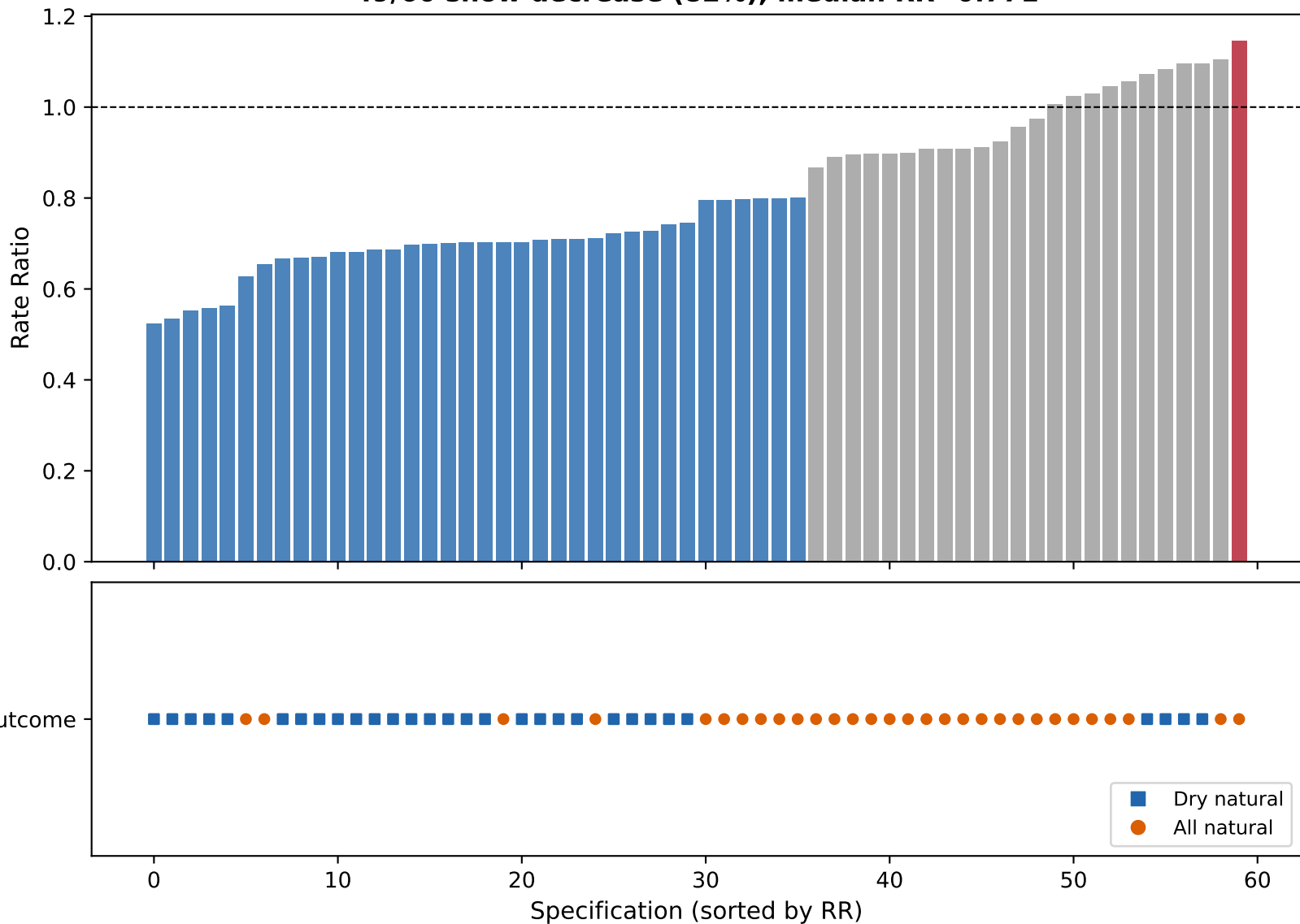
Figure 3: Specification Curve (60 Model Variants) 49/60 show decrease (82%), median RR=0.771
