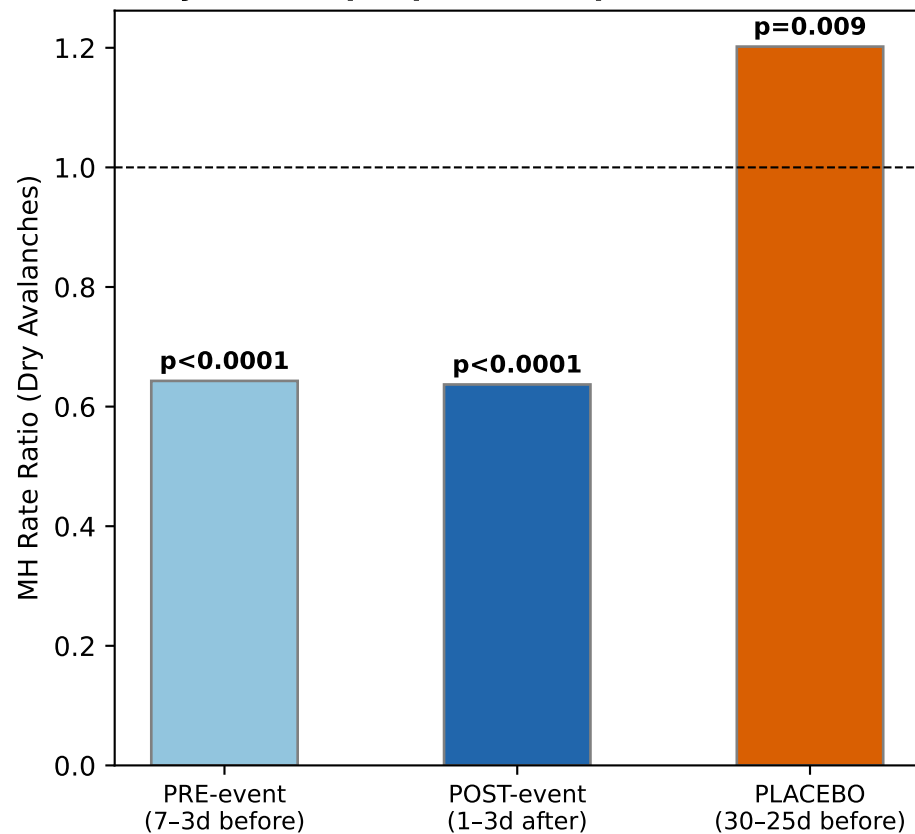
B: Geomag Events → Dry Avalanches (Symmetric pre/post = temporal association)
