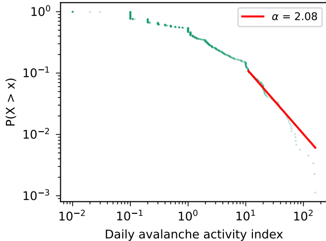
b Avalanches ( \alpha = 2.08 )
