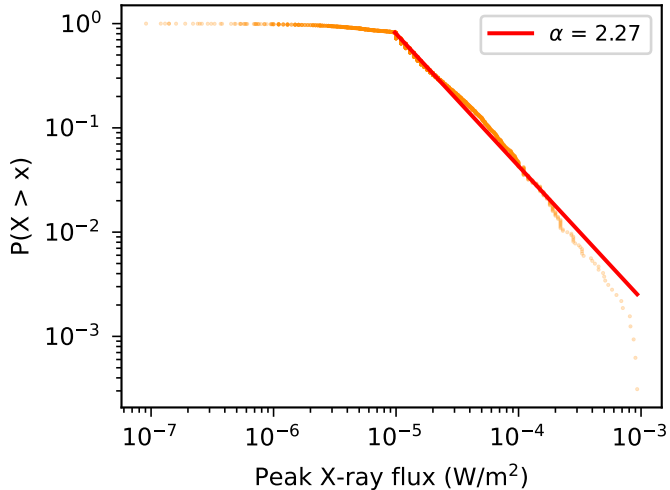
a Solar flares ( \alpha = 2.27 )
