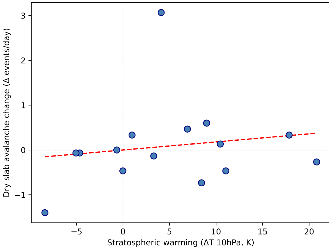
Event-by-Event: Stratospheric Warming vs Avalanche Response Pearson r=0.15 ( P=0.583 ), Spearman \rho=0.20 ( P=0.475 )
