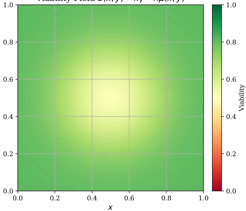
Viability Field b(x, y) = \kappa\gamma - \lambda\mu(x, y)
