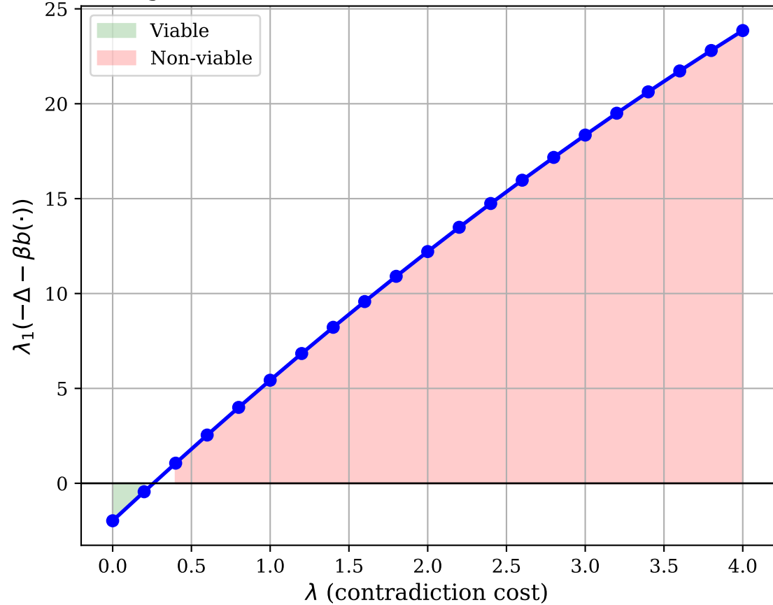
Eigenvalue Indicator Under Canonical Closure
