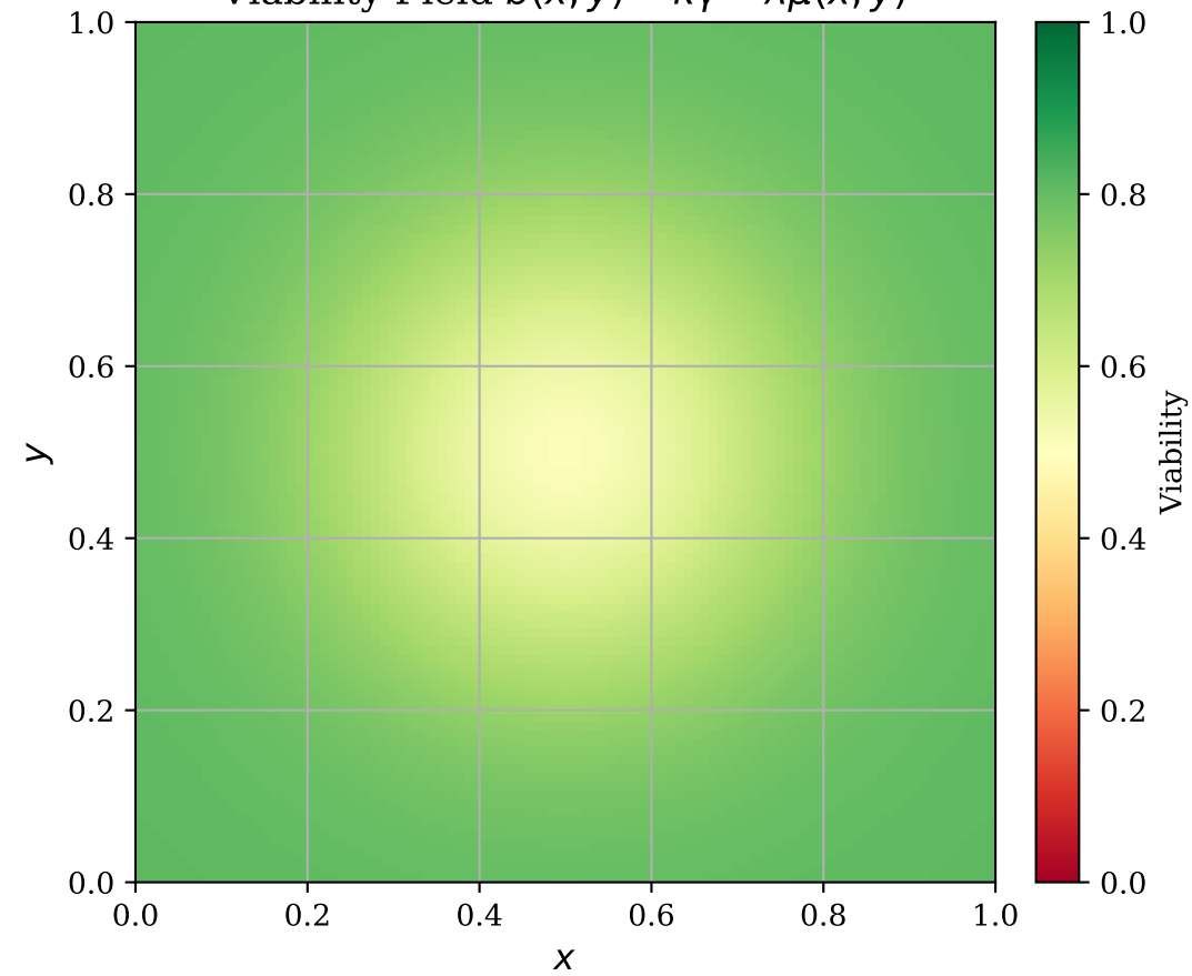
Viability Field b(x, y) = \kappa\gamma - \lambda\mu(x, y)
