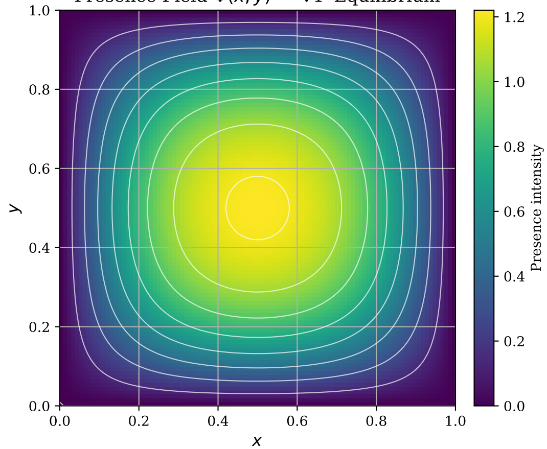
Presence Field \Phi(x, y) - V1' Equilibrium
