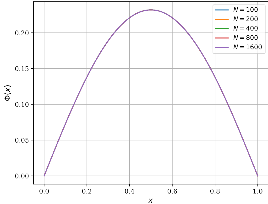
Solution Convergence Under Grid Refinement
