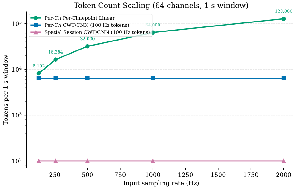
Figure 1: Token count scaling for a 1 s window with 64 channels. The per-timepoint linear tokenizer scales linearly with both sampling rate and channel count. CWT- and CNN-based tokenizers decouple token count from sampling rate; spatial projection further decouples it from channel count.
