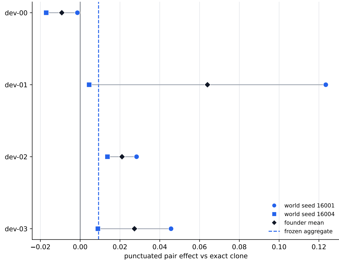
A R18 development (selected repeat) frozen aggregate = +0.009246
