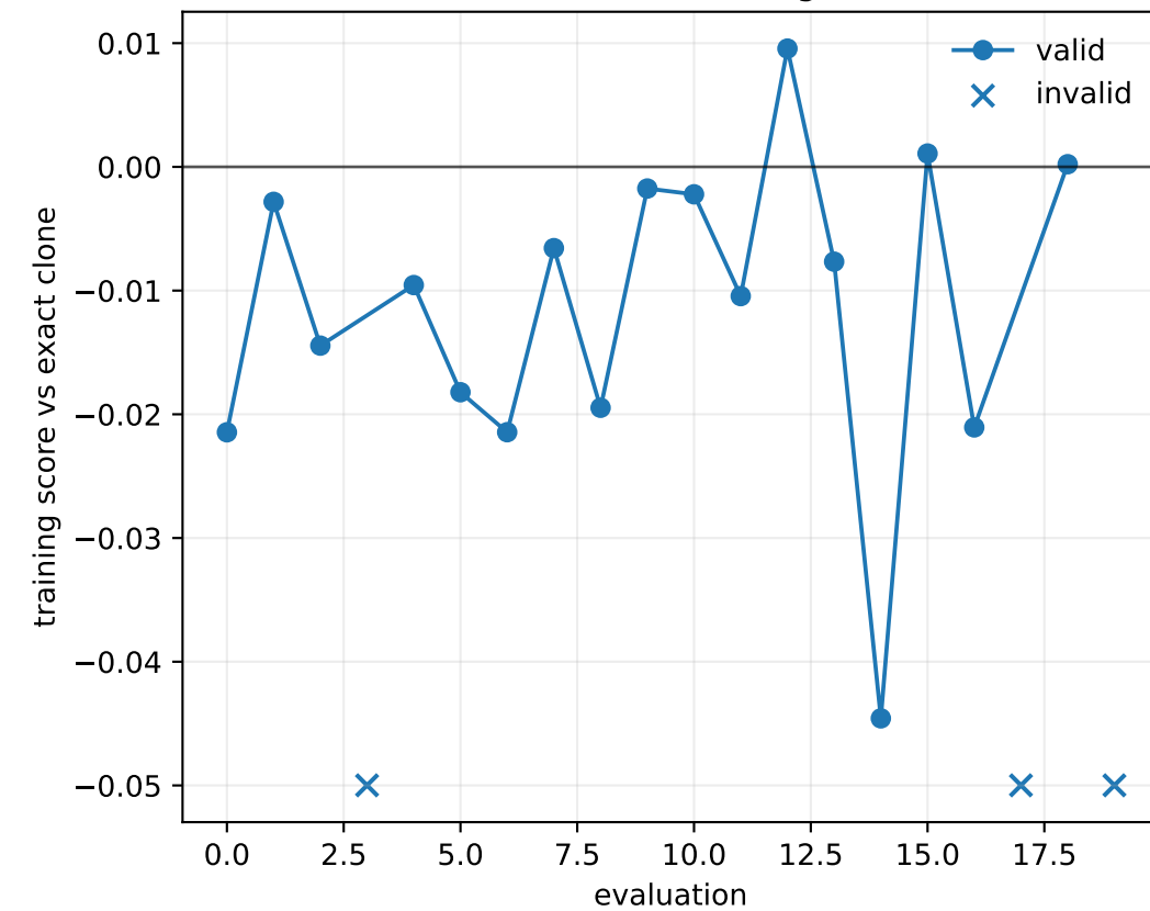
R15 Shinka lineage
