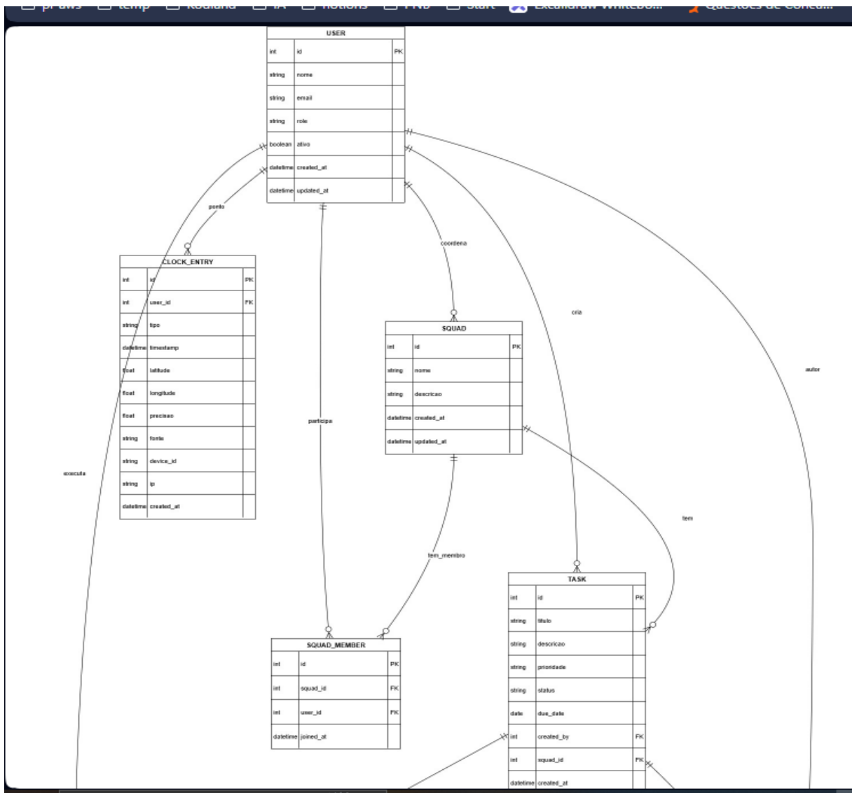
Figura 1 – Diagrama de Classes do Backend.
