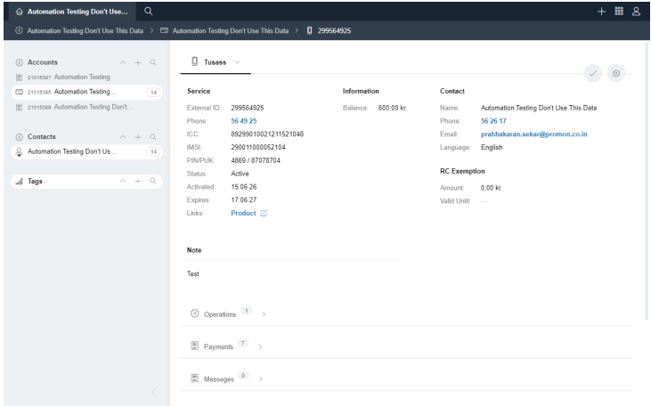
Screenshot 2
