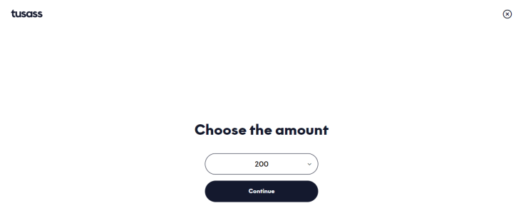
Screenshot 2
