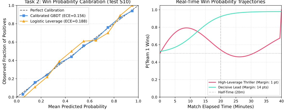
Figure 3: In-Game Win Probability Dynamics (Task 2). (Left) Reliability calibration curves on the out-of-sample Season 10 test set. (Right) Sample win probability trajectories comparing a tight comeback thriller against a decisive blowout.
