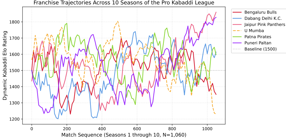
Figure 4: Franchise Elo Trajectories Across 10 Seasons (Task 3) . Dynamic ratings of leading PKL franchises from Season 1 to Season 10, capturing historical dynasty runs (e.g., Patna Pirates’ three-peat in Seasons 3–5).
