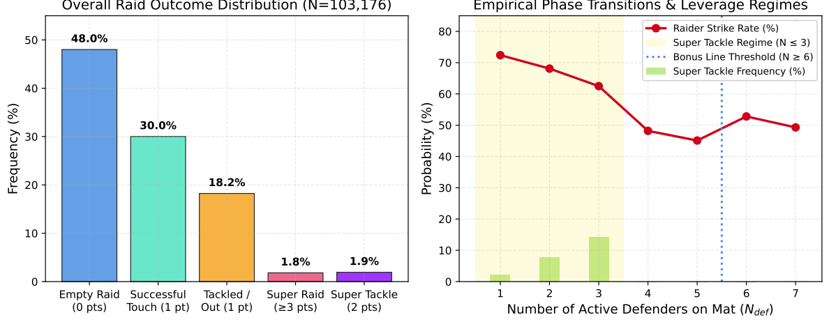
Figure 1: Strategic Phase Transitions in Kabaddi. (Left) Empirical distribution of raid outcome categories across 103,176 events in PKL-Bench. (Right) Raider strike rate and super tackle probability as a function of defender count N_{def} , highlighting the Bonus Line activation threshold ( N_{def} \geq 6 ) and the Super Tackle regime ( N_{def} \leq 3 ).
