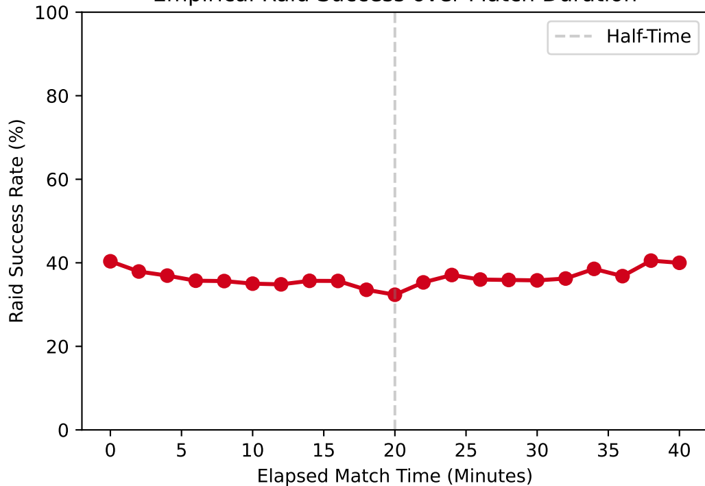
Empirical Raid Success over Match Duration
