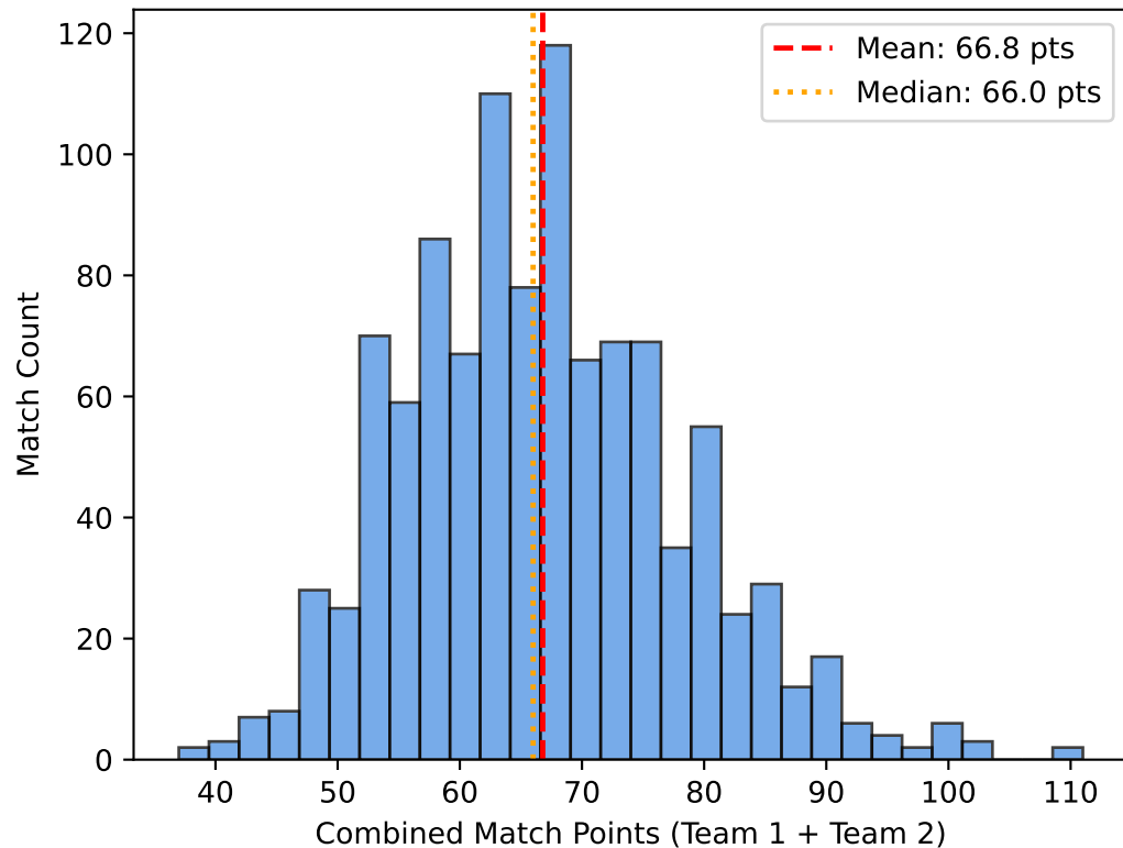
Total Scoring Distribution Across 1,060 Matches
