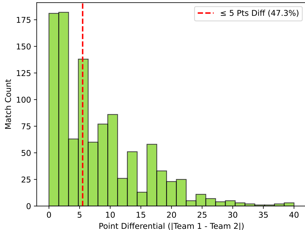
Margin of Victory Distribution
