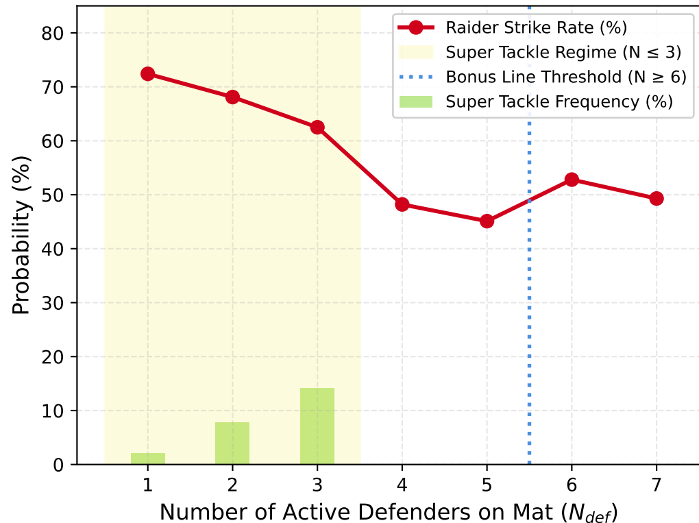
Empirical Phase Transitions & Leverage Regimes
