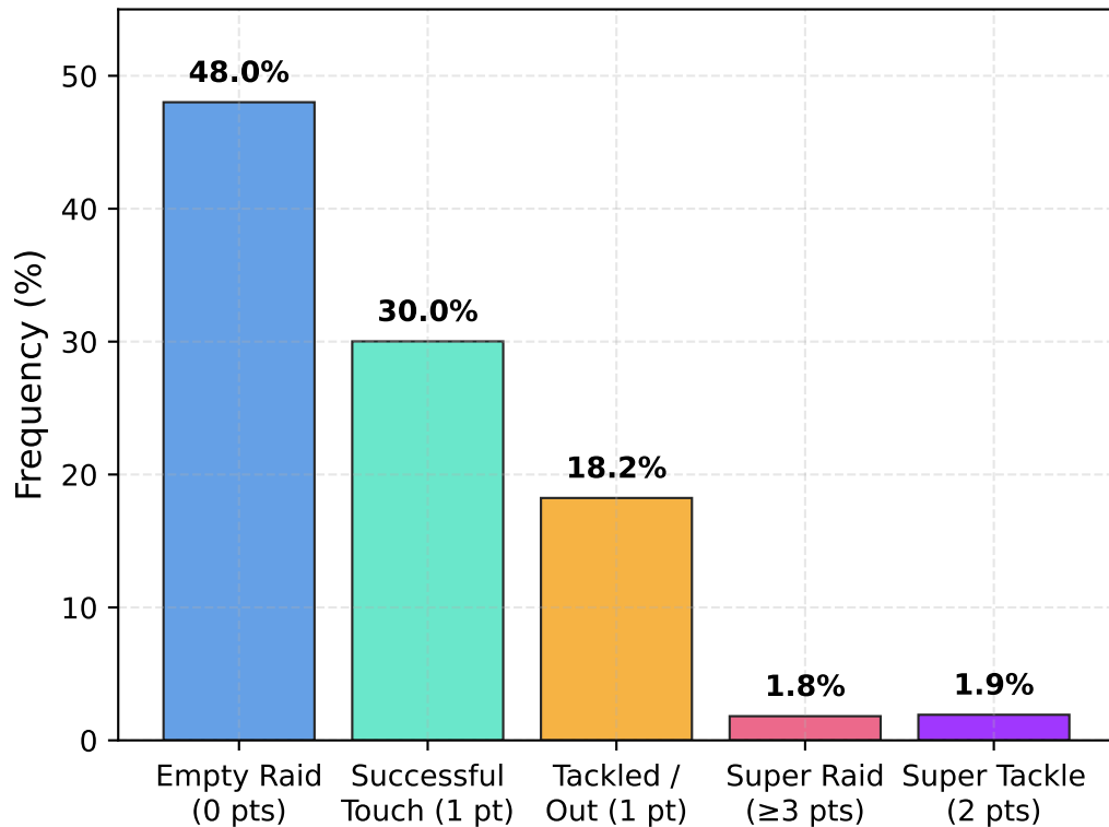
Overall Raid Outcome Distribution (N=103,176)
