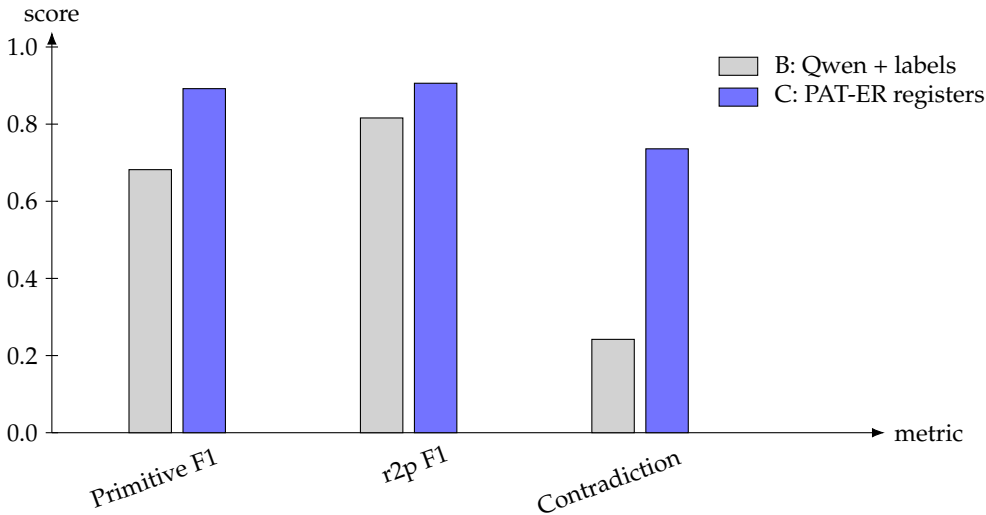
Figure 2. Contribution matrix graph. PAT-ER registers improve primitive macro-F1, role-to-primitive macro-F1, and contradiction recall over the token-pooled baseline on the same backbone.
