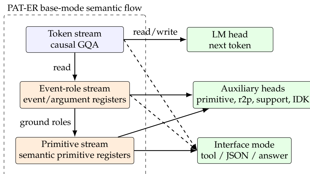
Figure 1. PAT-ER contains a normal token stream plus event-role and primitive side-state streams. The architecture claim is evaluated in base mode. Product-format generation is handled separately by the decoupled interface path.
