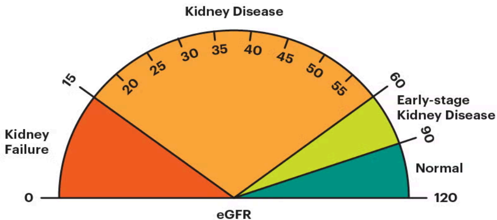
Fig 1: Physiological Range of eGFR(estimated GFR)( National Kidney Foundation )
