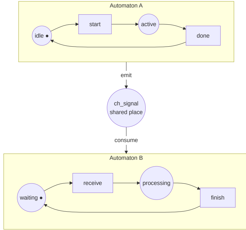
Figure 9.1: Two automata (A and B) lifted to Petri net subnets. The shared channel place ch_signal connects the output of automaton A to the input of automaton B.
