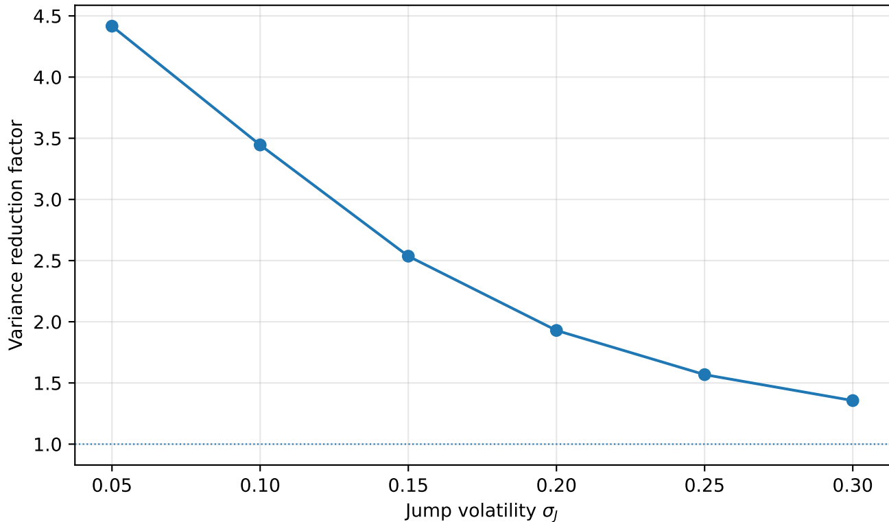
Control-Variate Efficiency vs Jump-Size Dispersion
