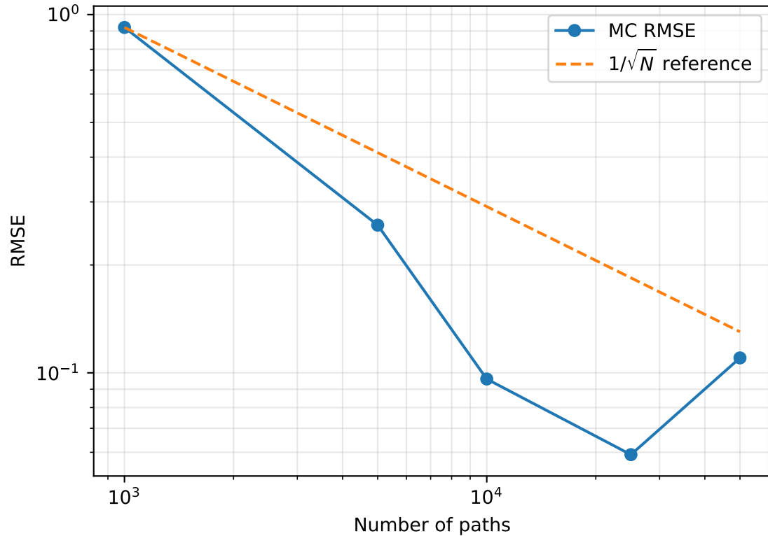
Convergence in Number of Paths
