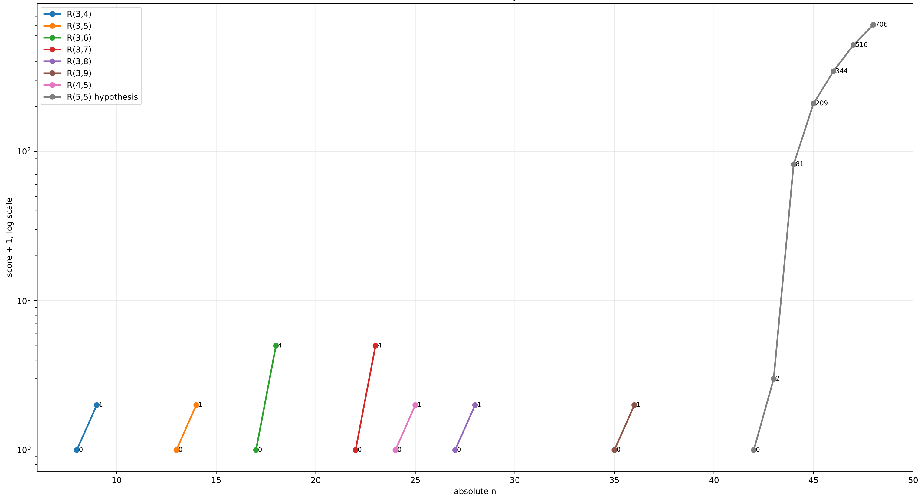
Theta and observed score by absolute n
