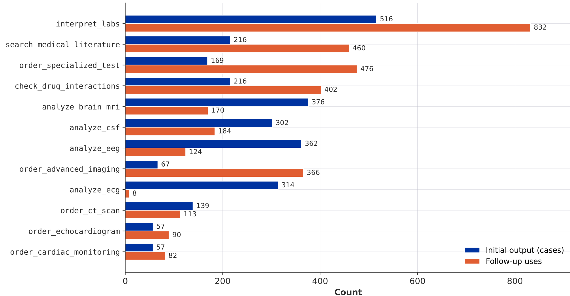
Tool output coverage (n = 516 cases, 12 tools)
