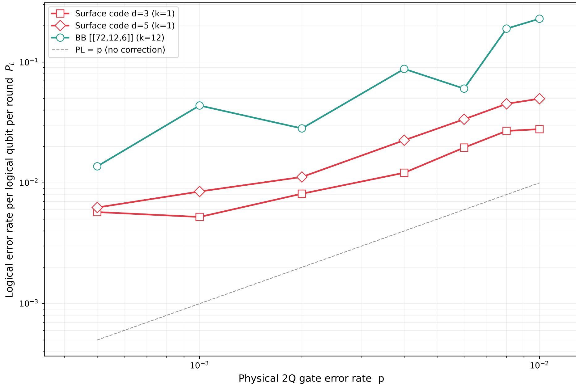
qLDPC vs Surface Code — Neutral Atom Platform (shuttling noise)
