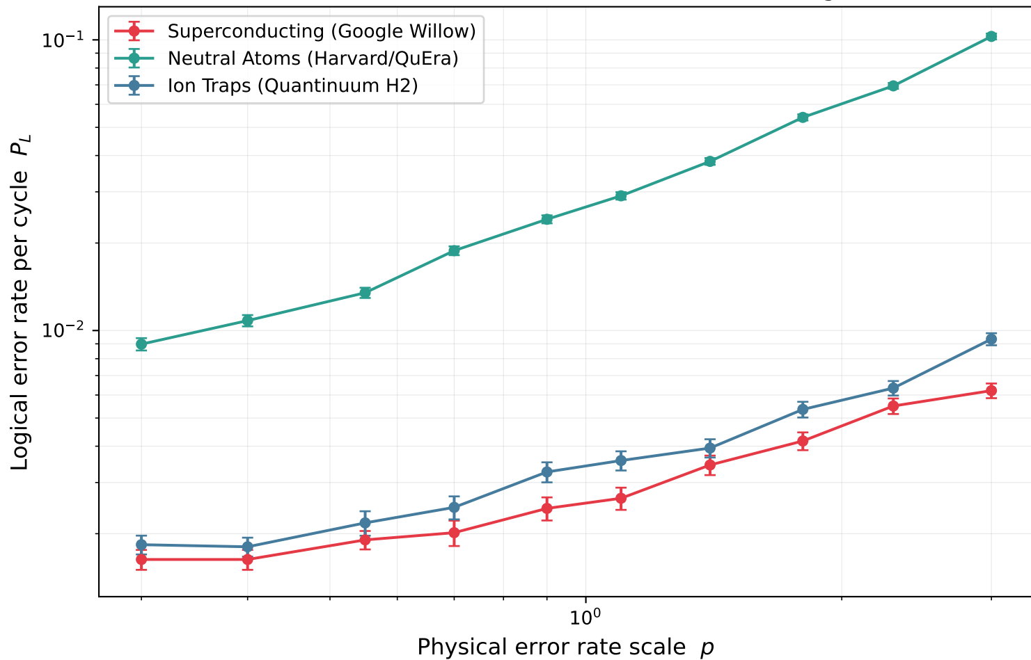
Surface code ( d=5 , R=5 ) — MWPM decoding
