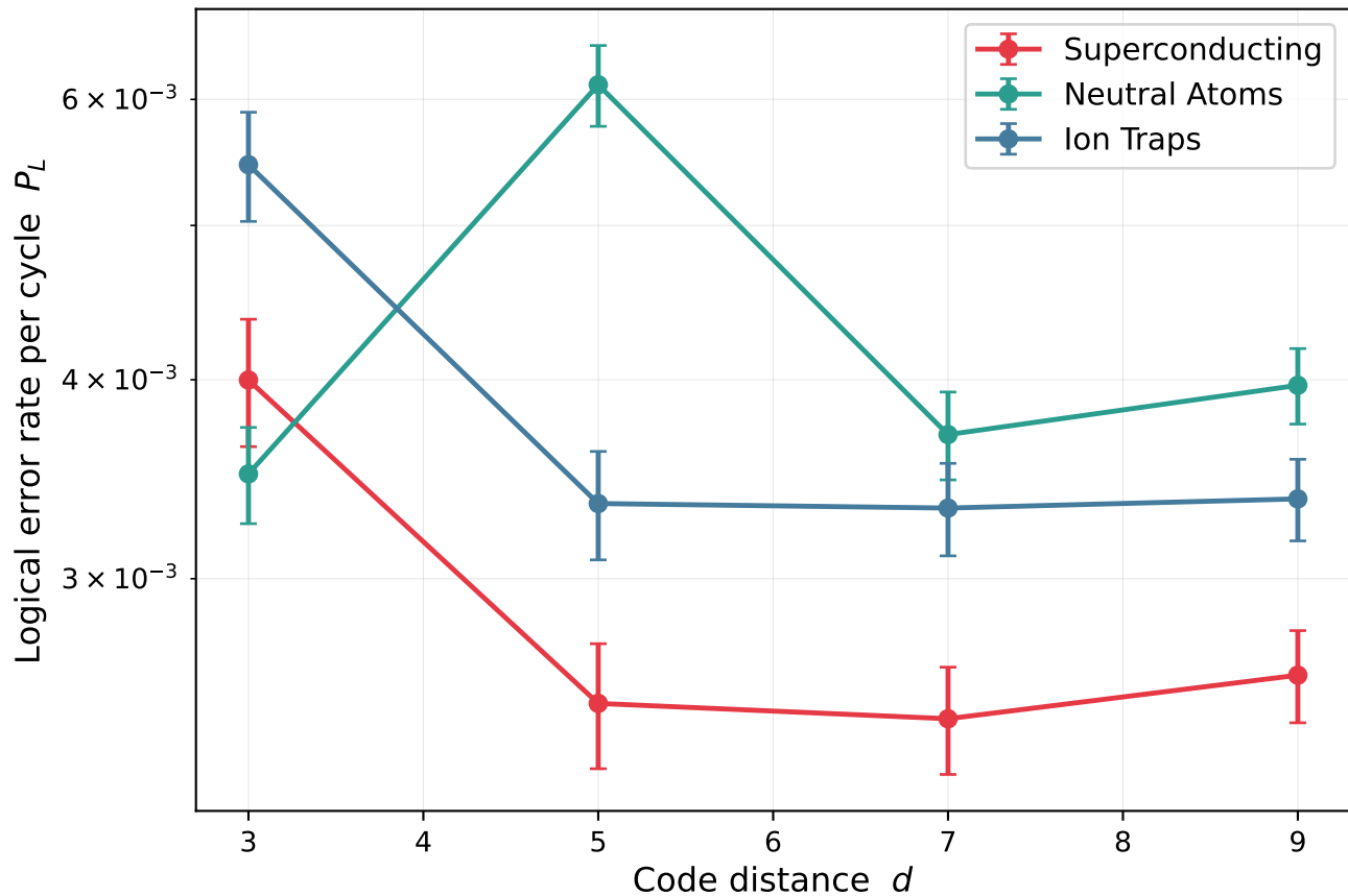
Error suppression: d vs PL ( p = 0.1\% , R = d )
