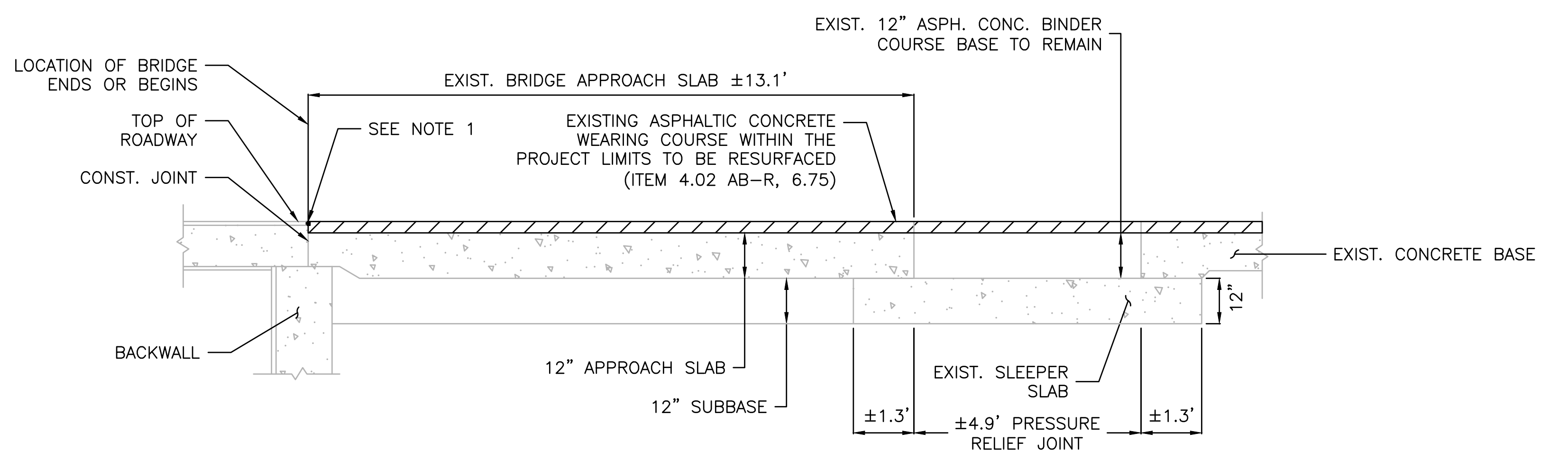
DETAIL #3 SECTION B-B: APPROACH SLAB AT GLENMORE AVENUE BRIDGE AND VAN SINDEREN AVENUE INTERSECTION LOOKING NORTH SCALE: N.T.S.
