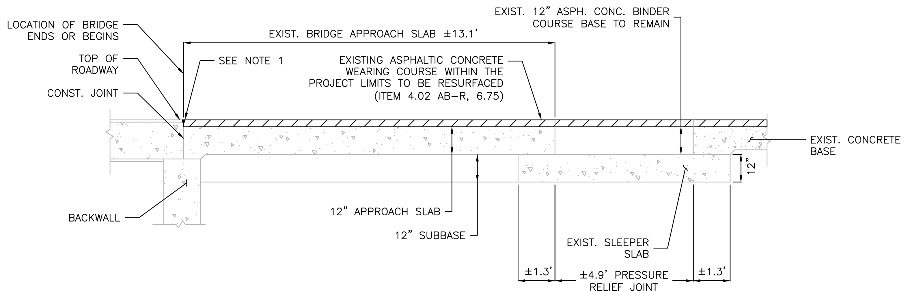
DETAIL #2 SECTION A-A: APPROACH SLAB AT LIBERTY AVENUE BRIDGE AND VAN SINDEREN AVENUE INTERSECTION LOOKING NORTH SCALE: N.T.S.
