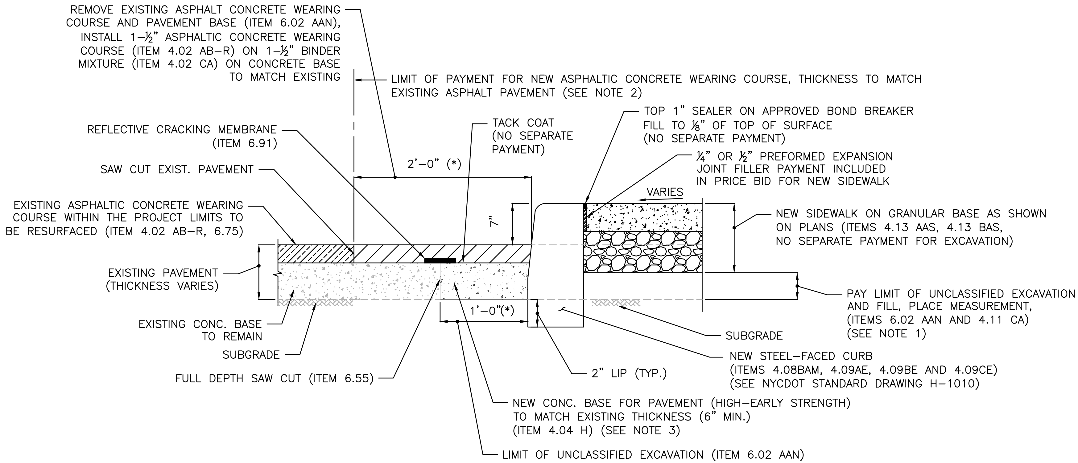
DETAIL #2 CURB, SIDEWALK, AND PAVEMENT DETAIL SCALE: N.T.S.
