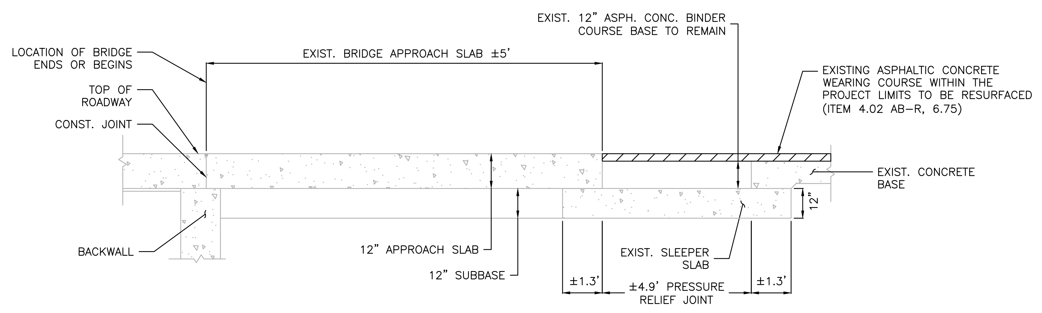
DETAIL #4 SECTION C-C: APPROACH SLAB AT PITKIN AVENUE BRIDGE AND VAN SINDEREN AVENUE INTERSECTION LOOKING NORTH SCALE: N.T.S.
