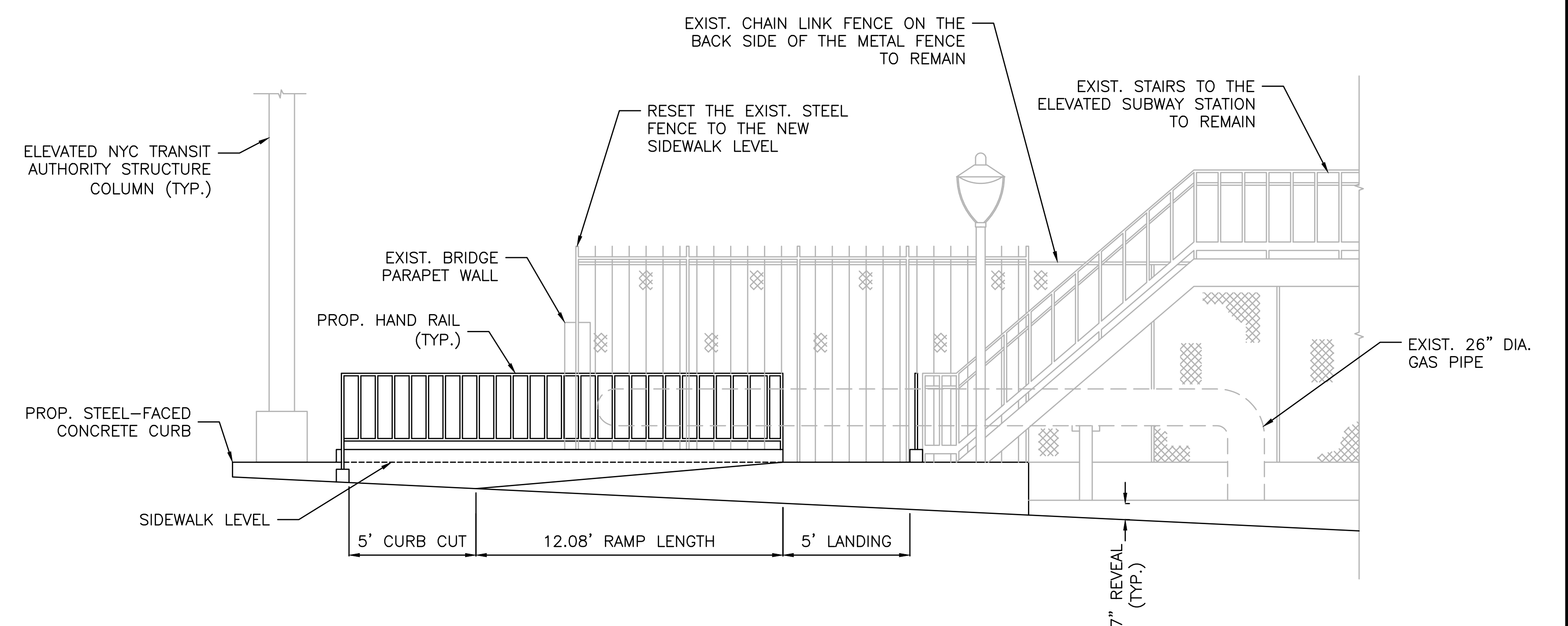
SECTION B-B
