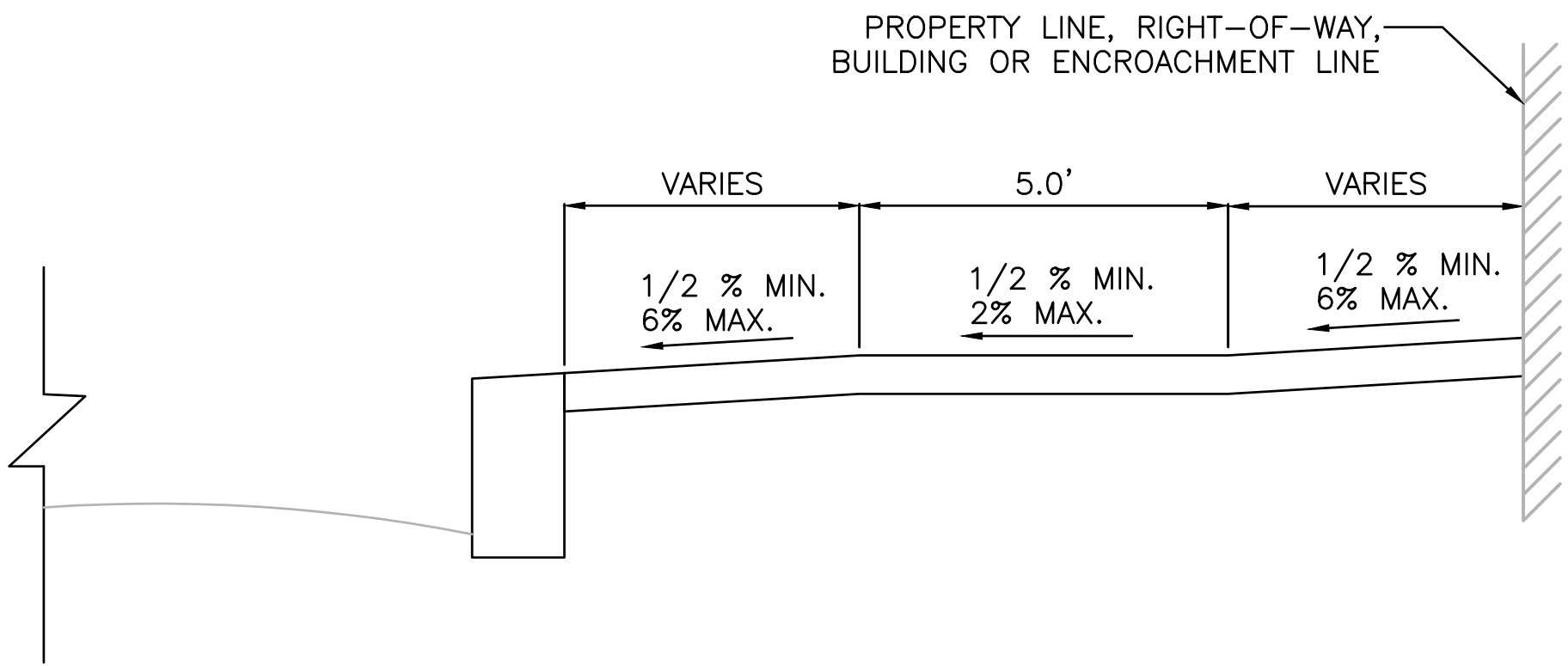
DETAIL #4 TYPICAL FULL WIDTH SIDEWALK SECTION ADA COMPLIANCE SCALE: N.T.S.
