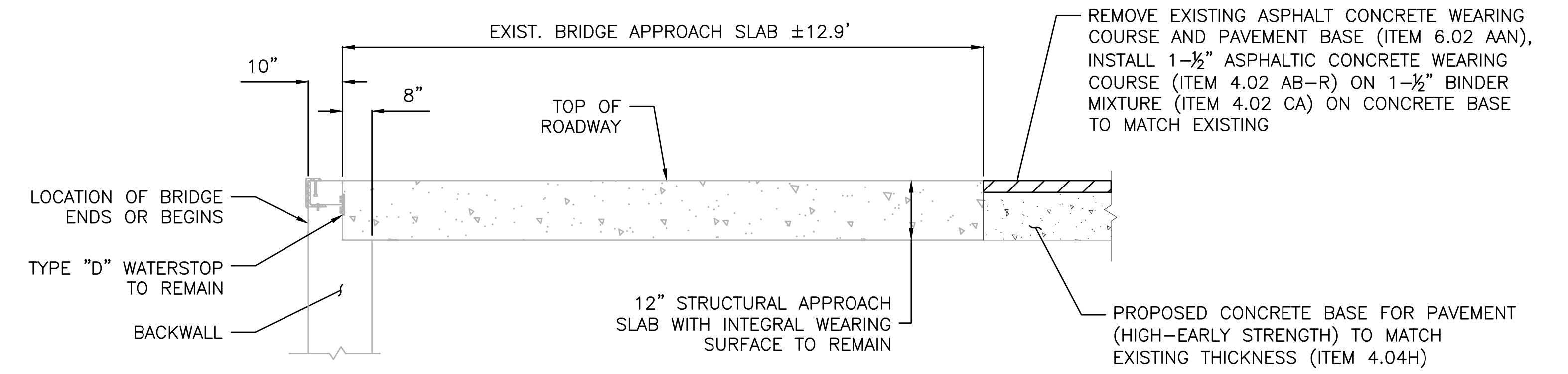
DETAIL #5 SECTION D-D: APPROACH SLAB AT SUTTER AVENUE BRIDGE AND VAN SINDEREN AVENUE INTERSECTION LOOKING NORTH SCALE: N.T.S.
