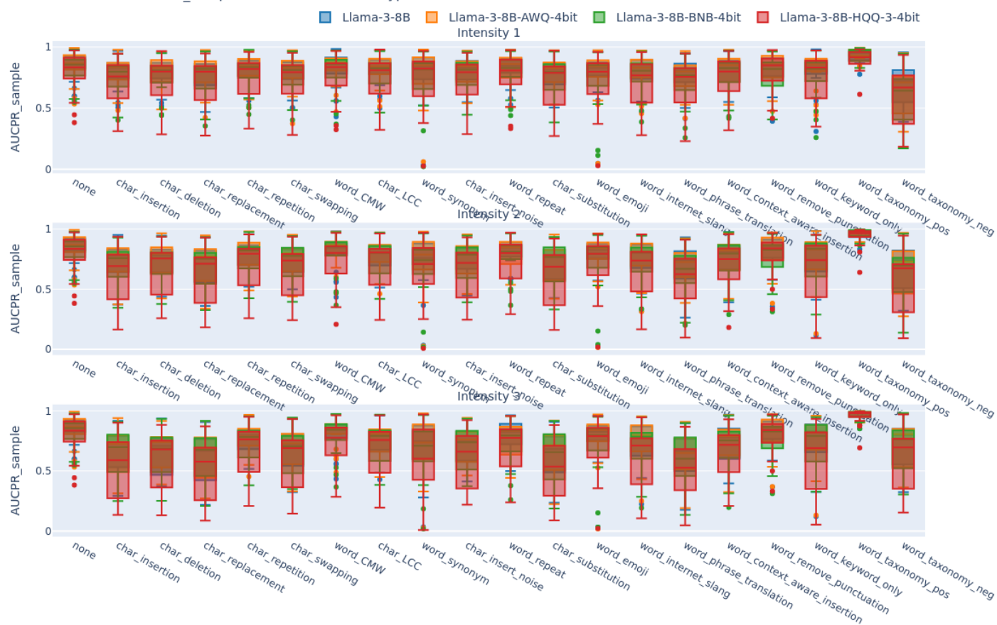
Distribution of AUCPR sample Across Perturbation Types
